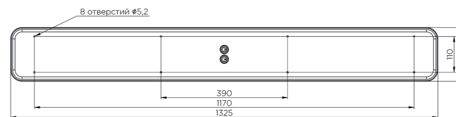
KLM61 2100 LED
